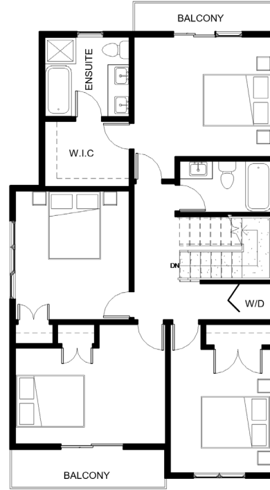
MAIN FLOOR
