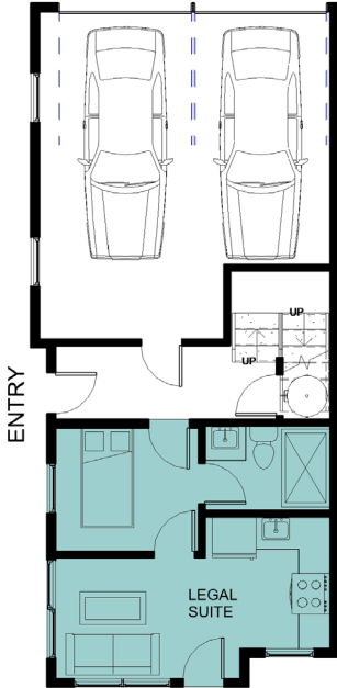
LOWER FLOOR
