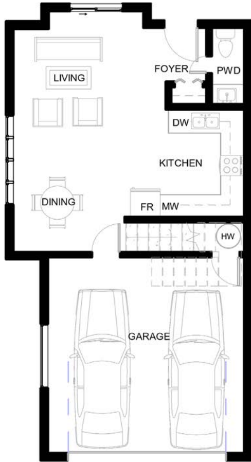
MAIN FLOOR
