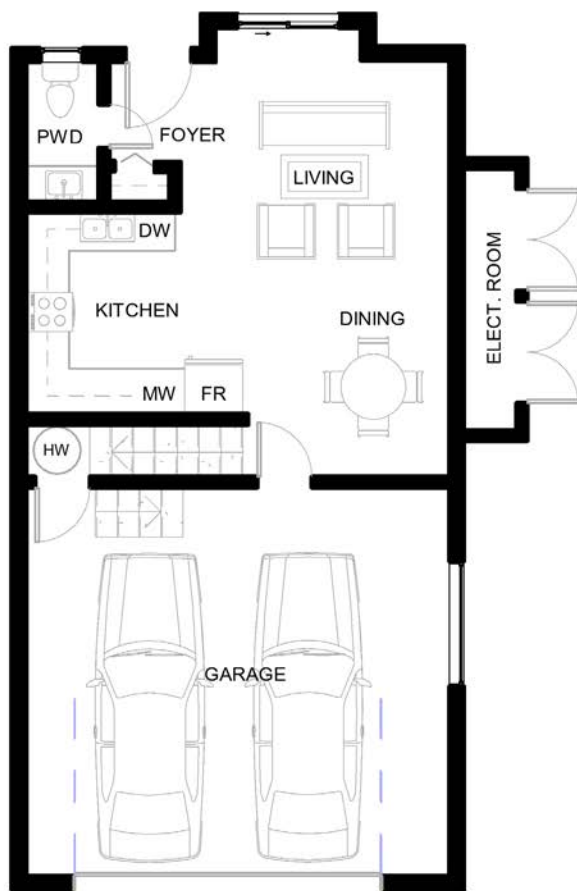
MAIN FLOOR
