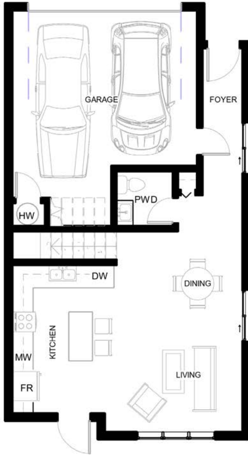
MAIN FLOOR
